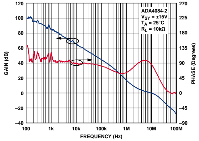
Figure 63. Open-Loop Gain and Phase vs. Frequency
