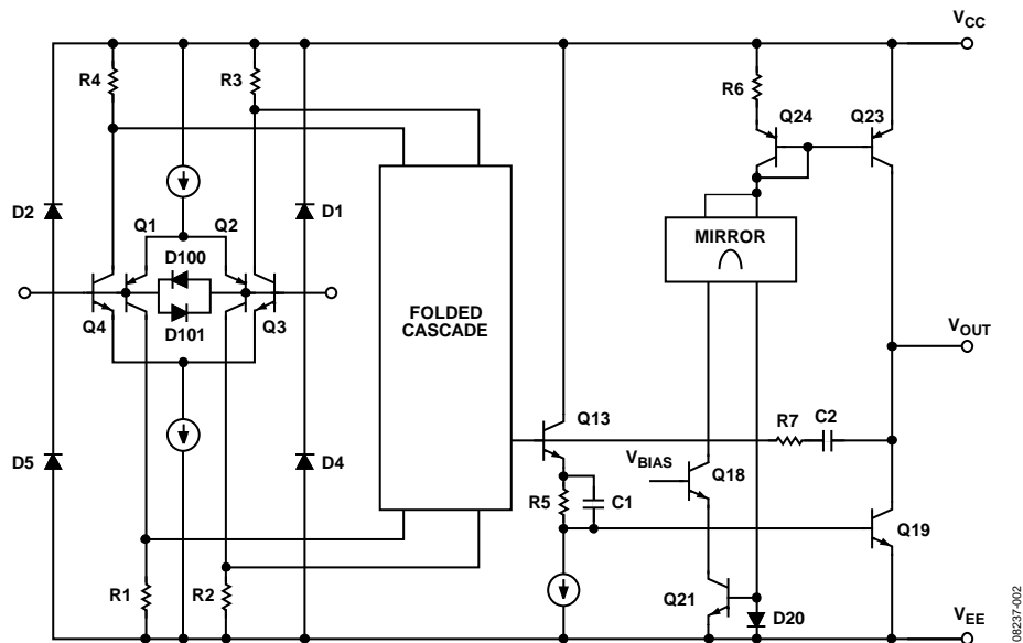
Figure 2. Simplified Schematic
