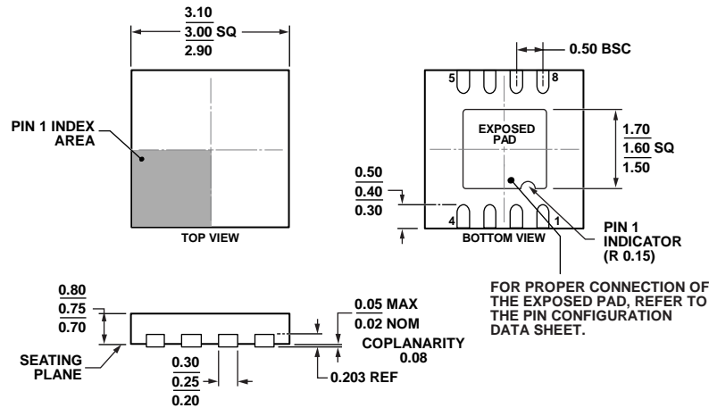
Figure 87. 8-Lead Lead Frame Chip Scale Package [LFCSWP_WD] 3 x 3 mm Body, Very Very Thin, Dual Lead (CP-8-12) Dimensions shown in millimeters
