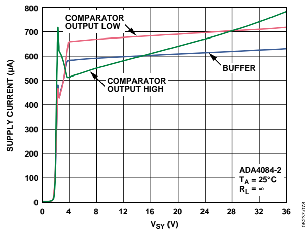
Figure 84. Supply Current vs. Supply Voltage
